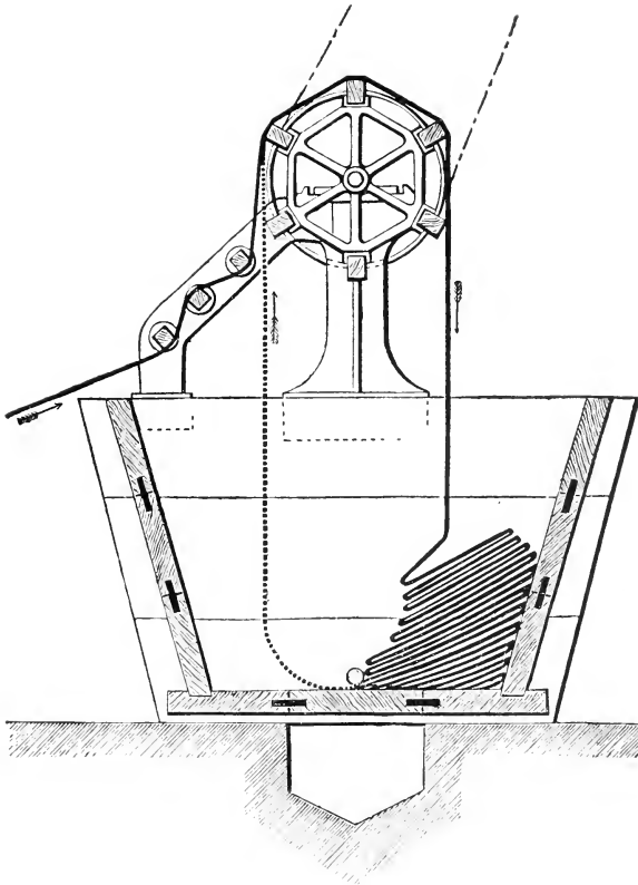
FIG. 20.—Jig Wince.
